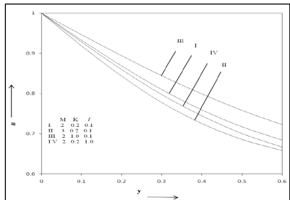
Fig 7.2: The Velocity Profiles of Fluid for Different Value of M , K and l .
